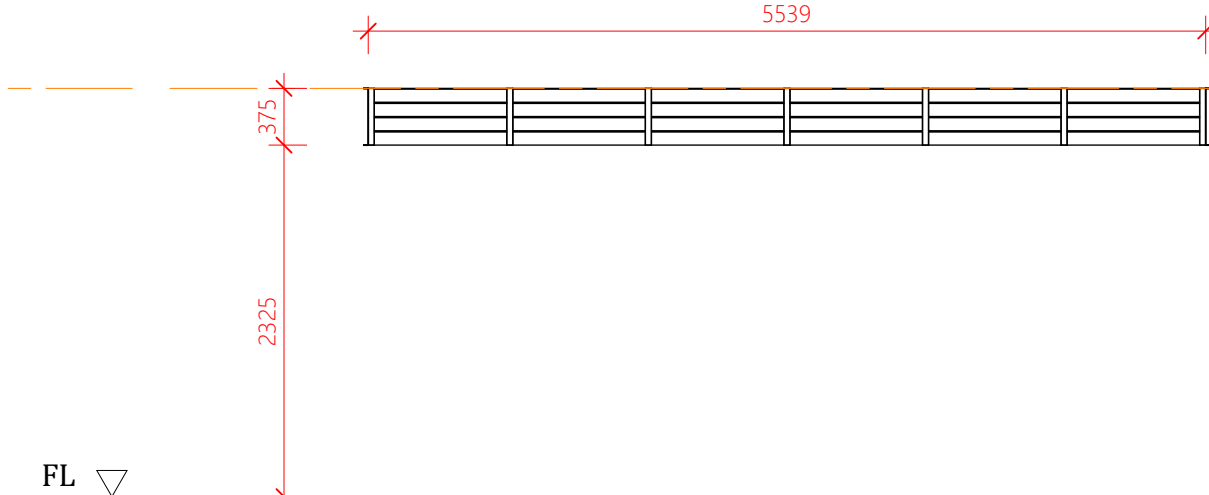
WINDOW TYPE I
