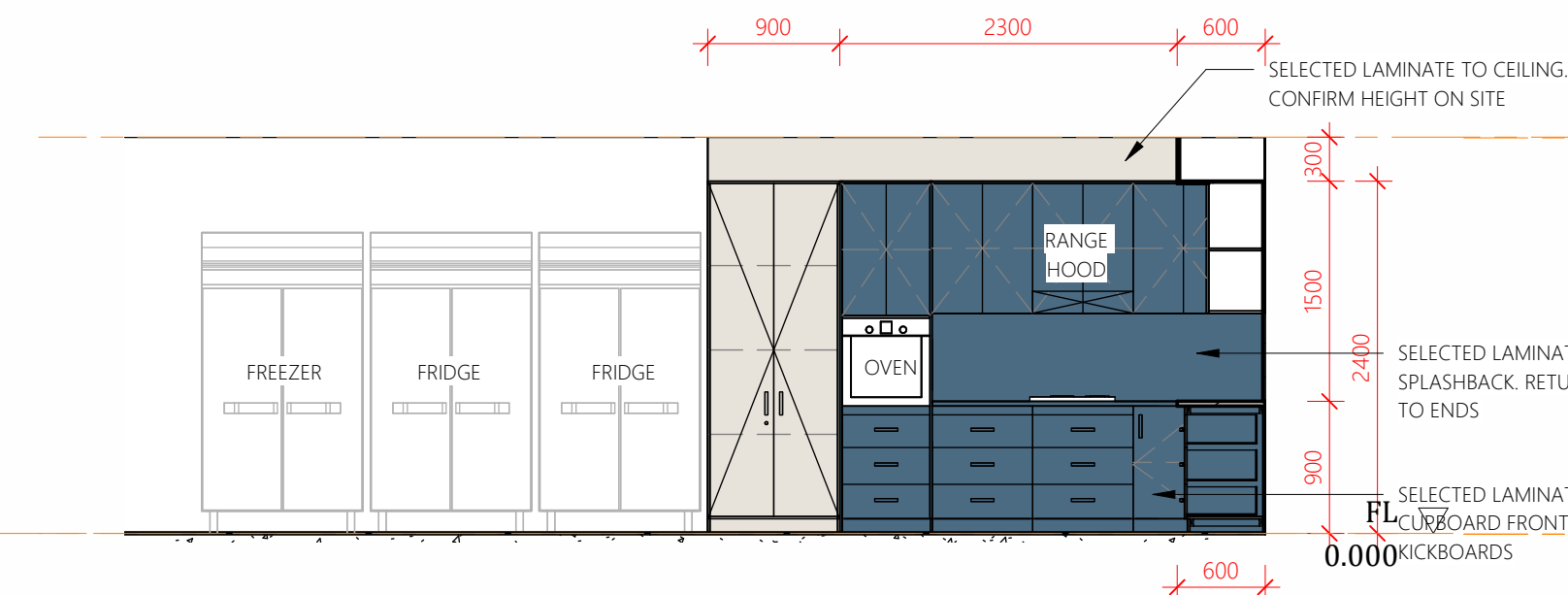
Elevation 2C
