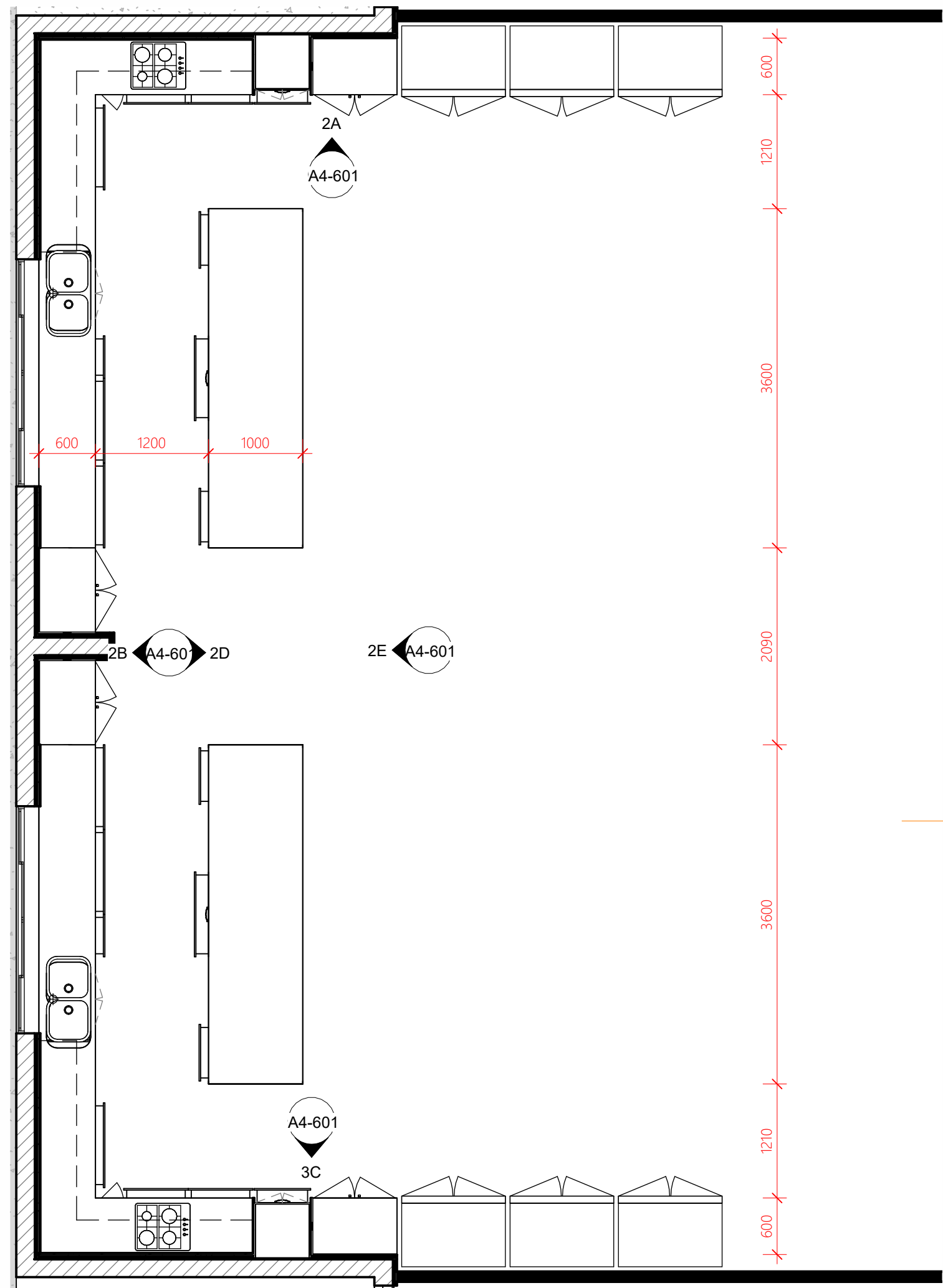
Internal Plan 1 - Kitchen
