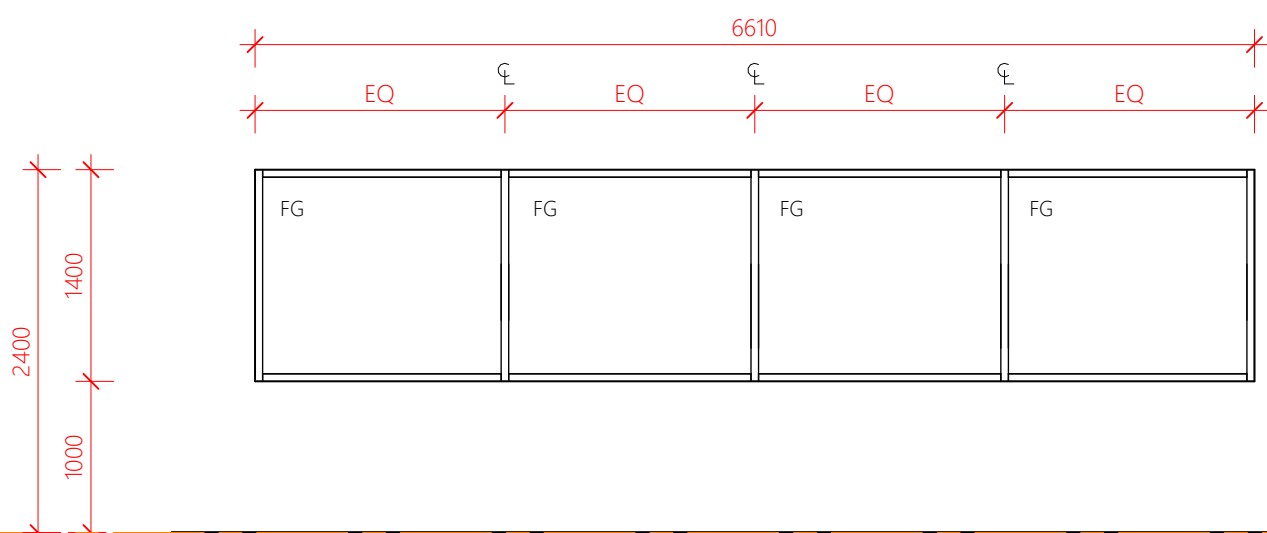
WINDOW TYPE A
