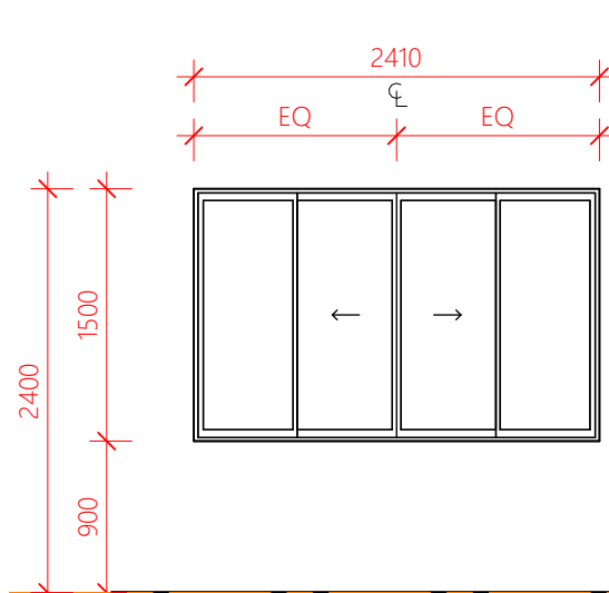
WINDOW TYPE E
