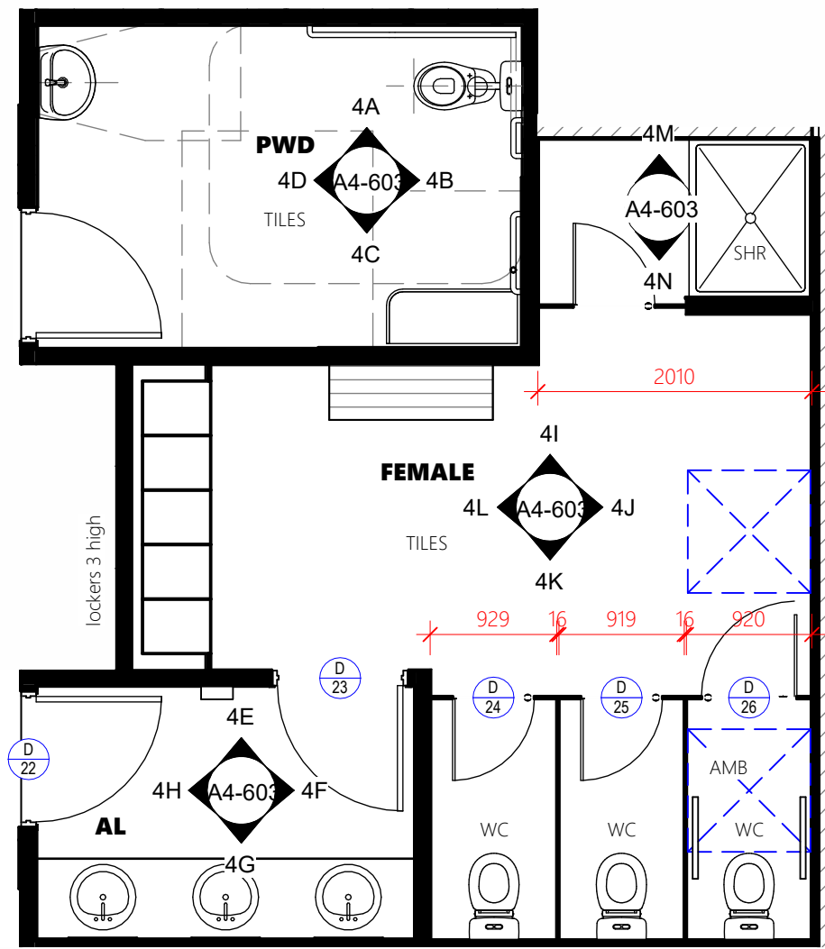
Internal Plan 3 - Amenities
