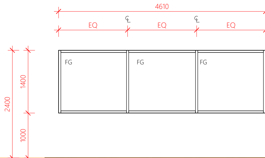
WINDOW TYPE B
