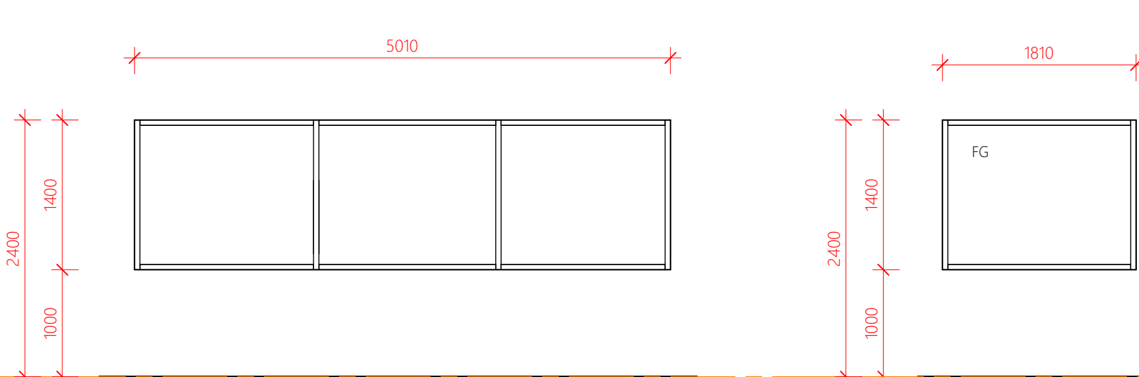
WINDOW TYPE C
